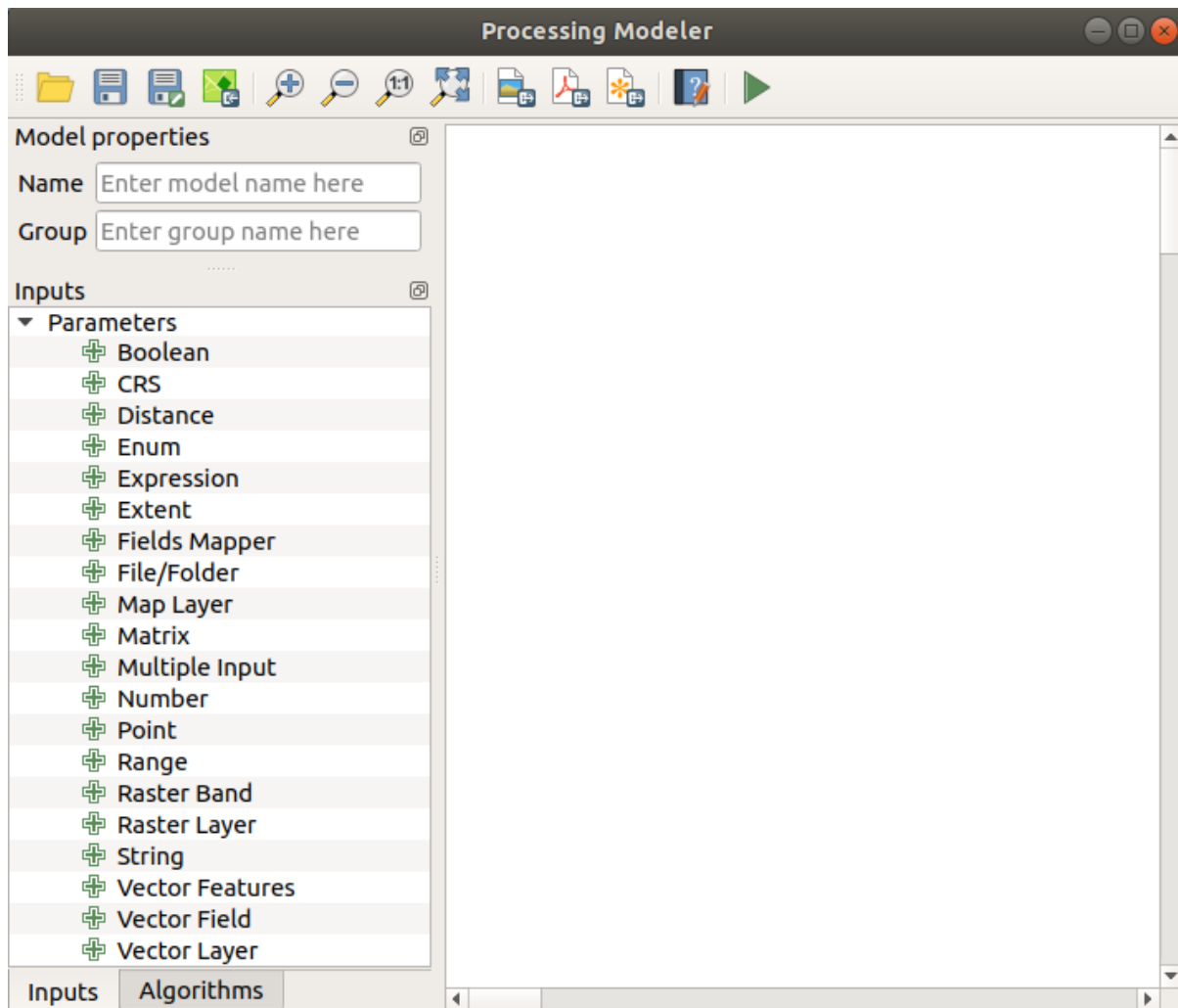
Fig. 21.18: Modeler
