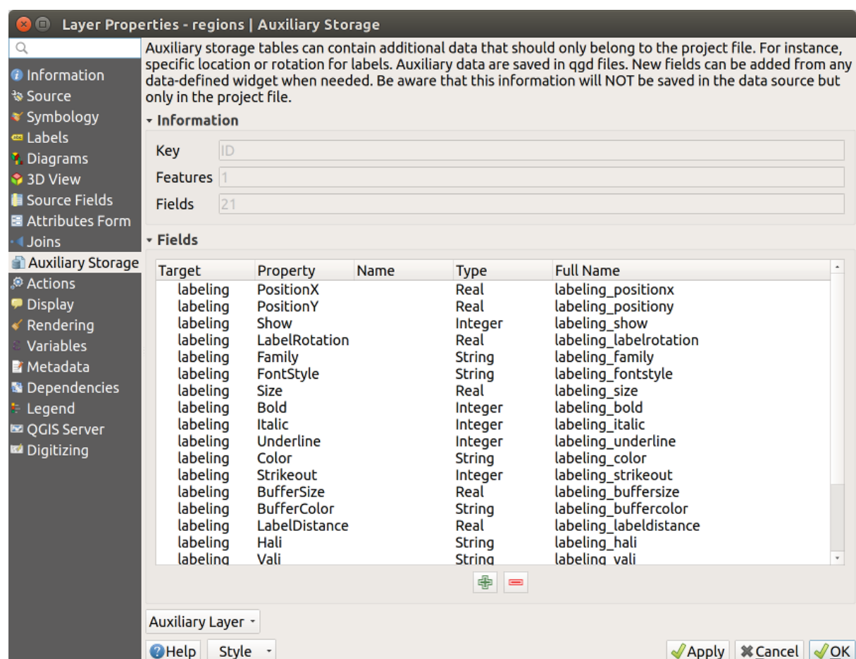
Fig. 13.57: Auxiliary Fields
