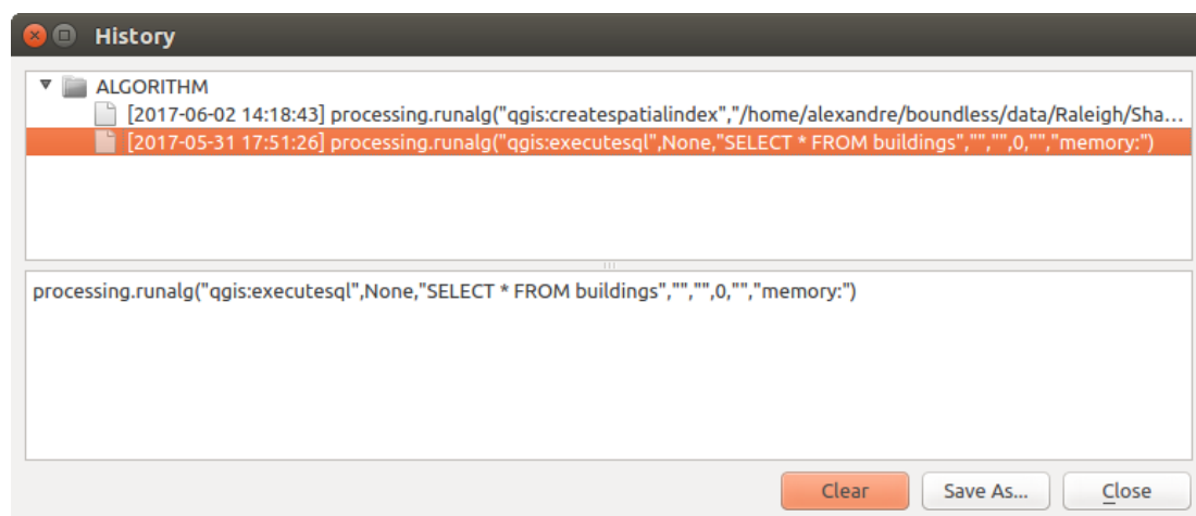
Fig. 21.17: History
