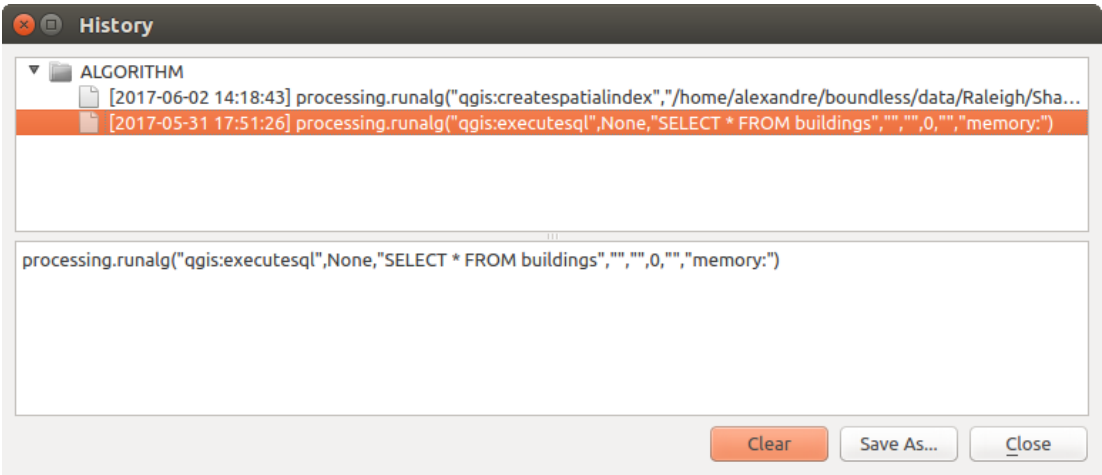
Fig. 21.3: Processing History
