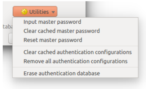
Fig. 19.15: Utilities menu
