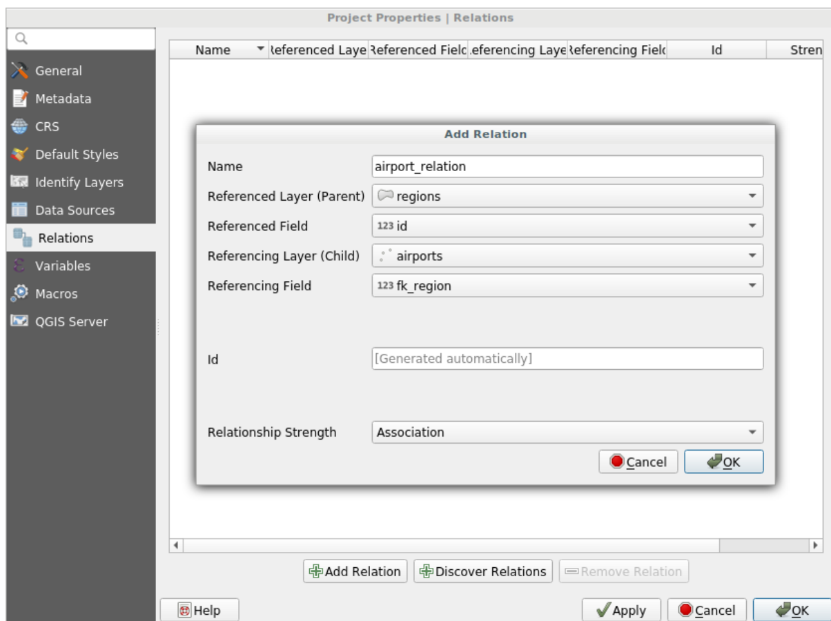
Fig. 13.85: Relation Manager
