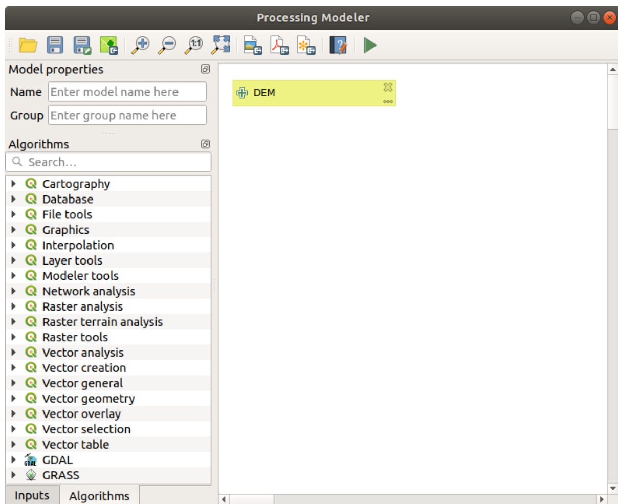
Fig. 21.21: Model Inputs
