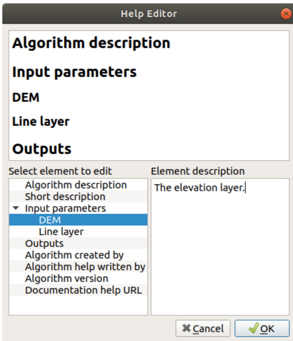
Fig. 21.27: Editing Help
