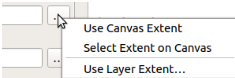
Fig. 21.11: Extent selector
