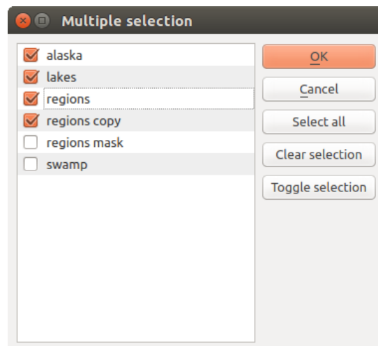
Fig. 21.14: Multiple Selection
