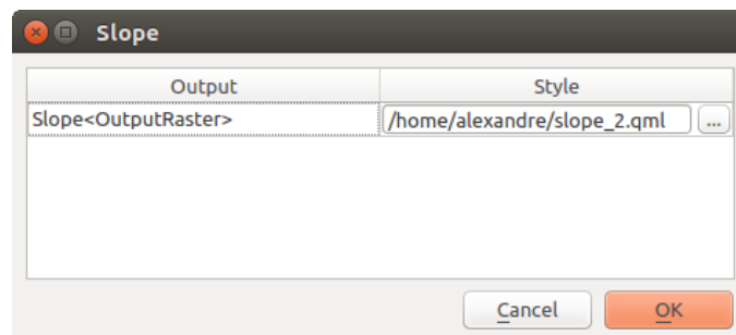
Fig. 21.5: Rendering Styles
