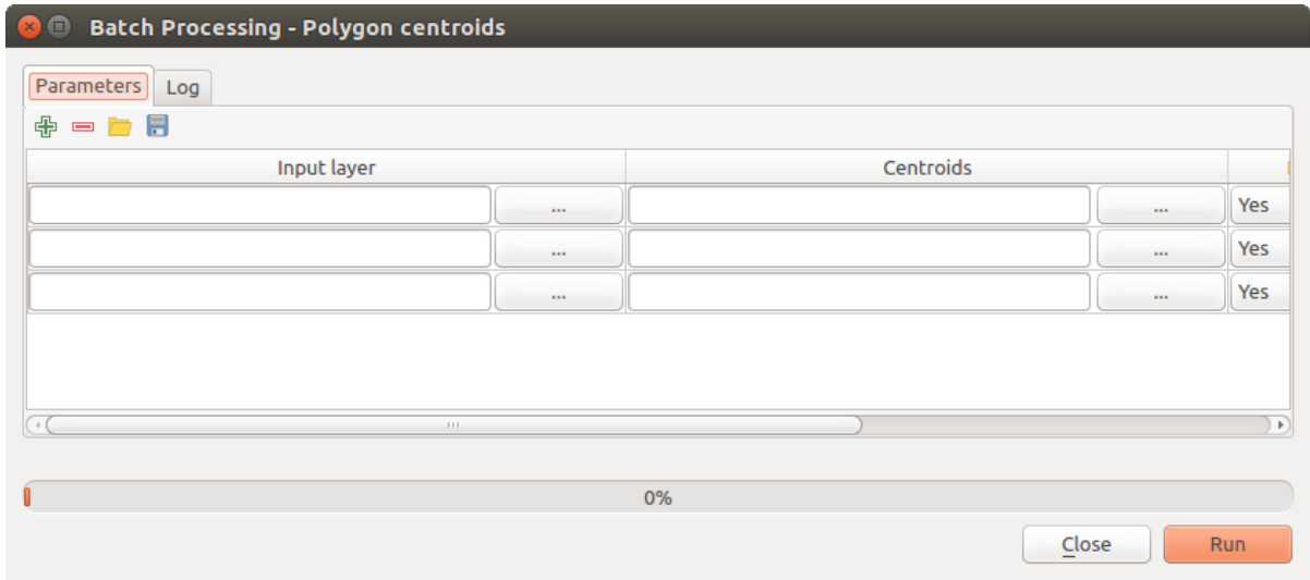
Fig. 21.30: Batch Processing
