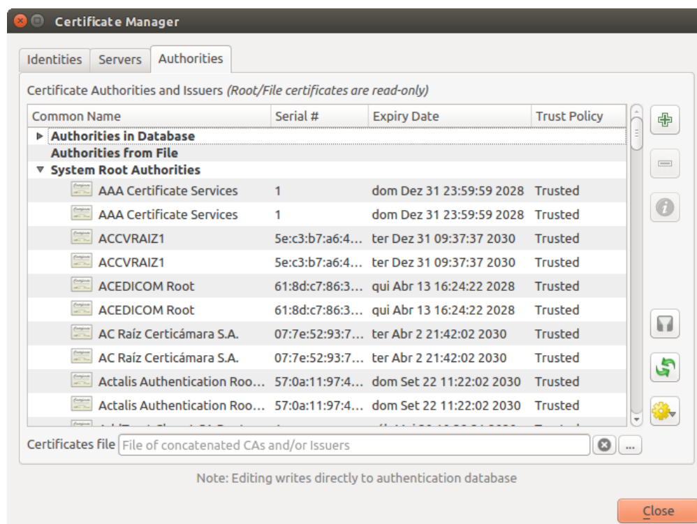
Fig. 19.24: Authorities editor
