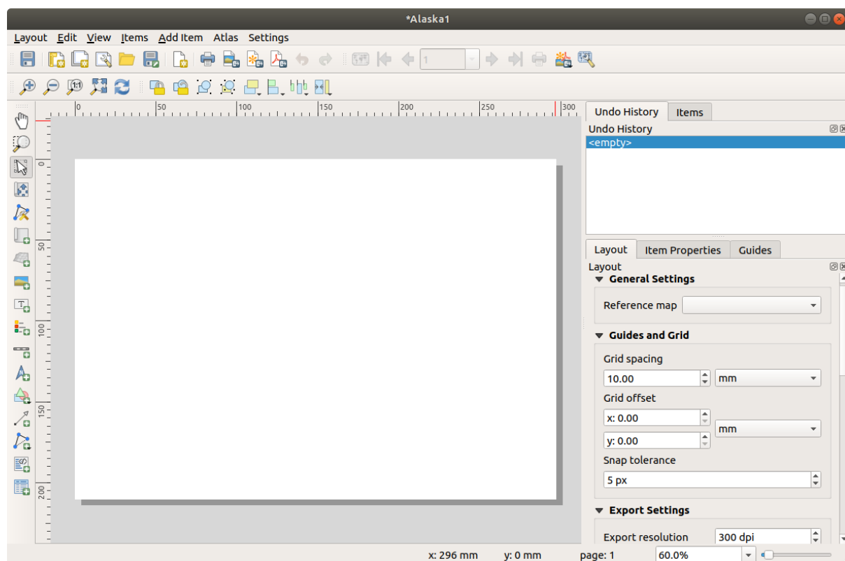
Fig. 16.2: Print Layout
